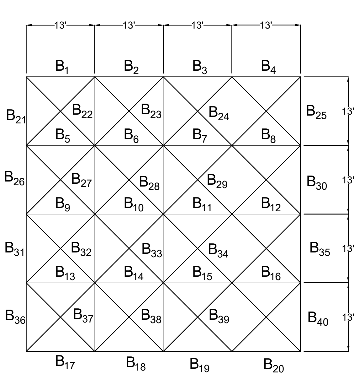
Yield Line Diagram
